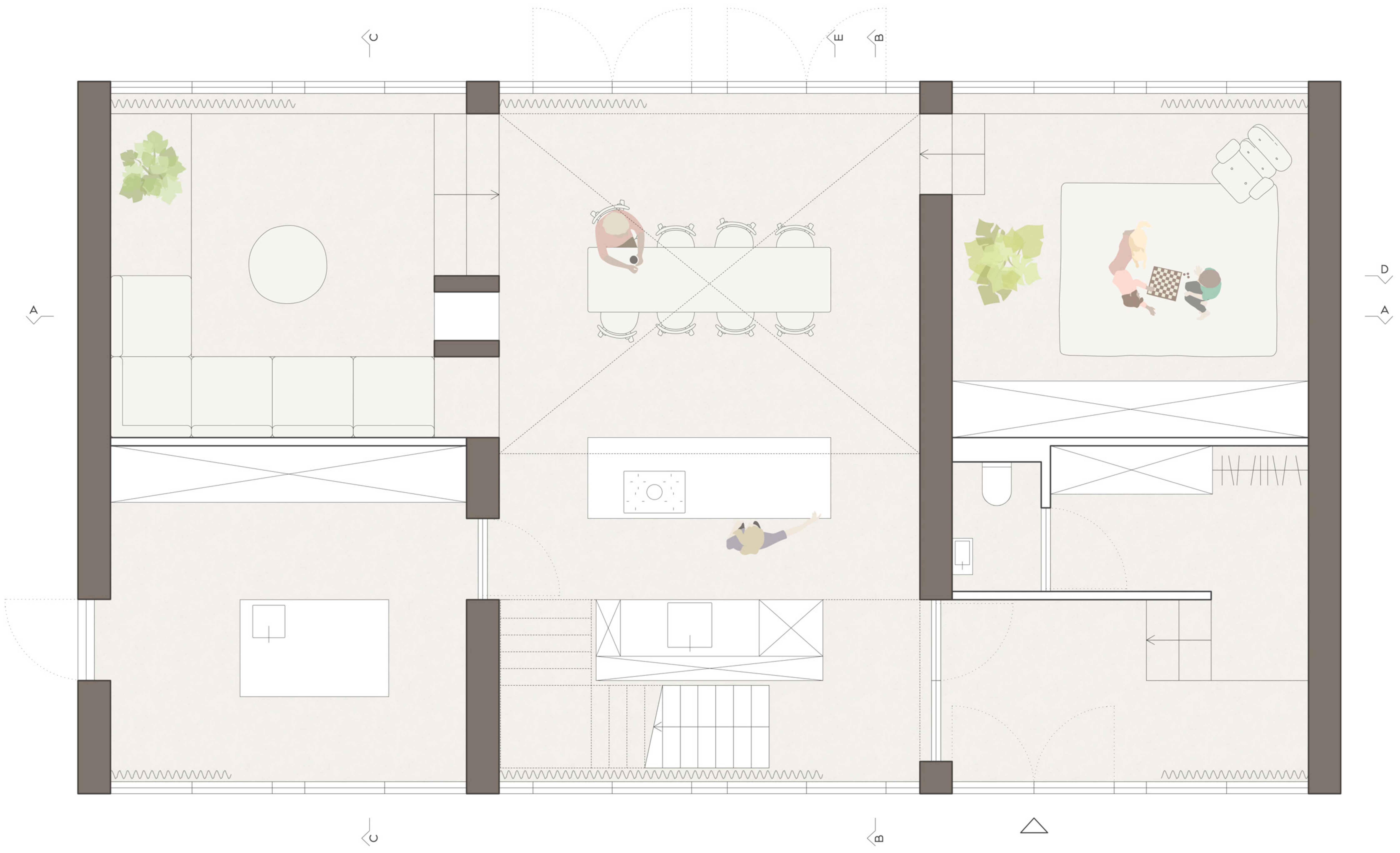
ground floor
